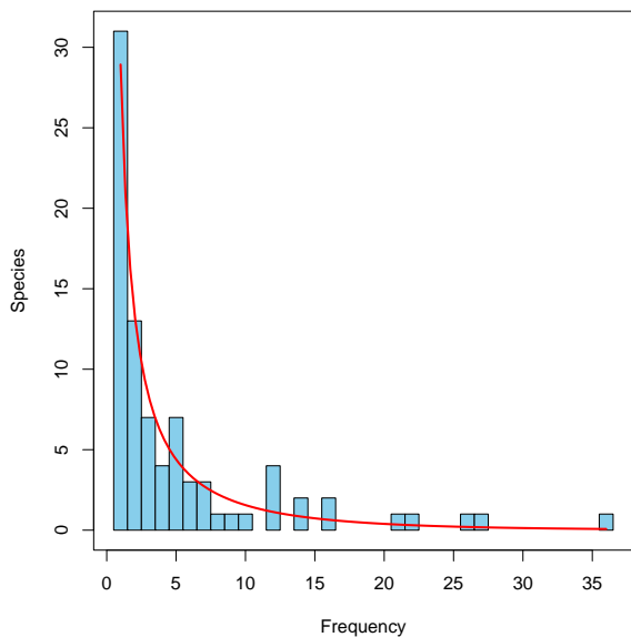
Figure 3: Fisher’s log-series fitted to one randomly selected site (2).
