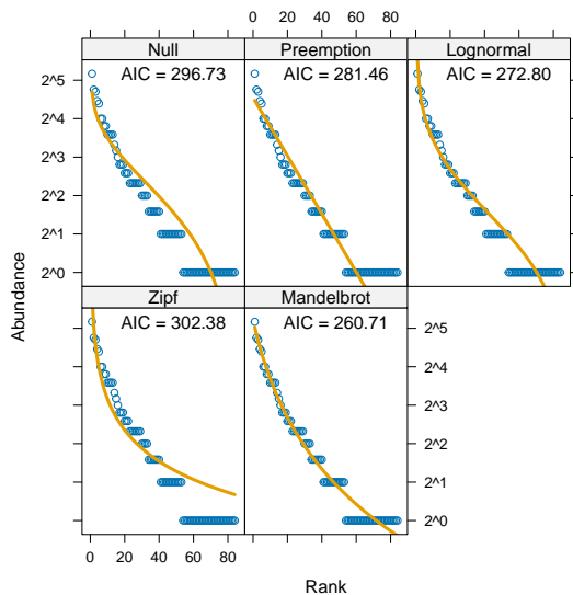
Figure 4: Ranked abundance distribution models for a random plot (no. 2). The best model has the lowest AIC.
